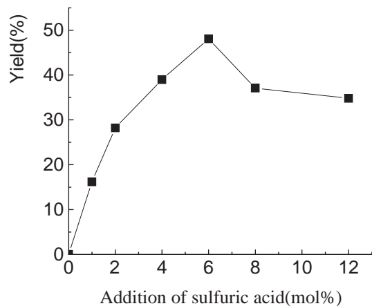
Fig. 1. Influence of \text{H}_2\text{SO}_4 concentration in the amidocarbonylation catalyzed by Pd/HZSM-5. Reaction conditions: 30 mmol isovaleraldehyde and amide, 60 mL NMP, 1.0 mol % Pd/HZSM-5, and 35 mol % LiBr were treated with 6.0 MPa CO at 90 °C for 16 h, without addition of \text{PPh}_3 .
